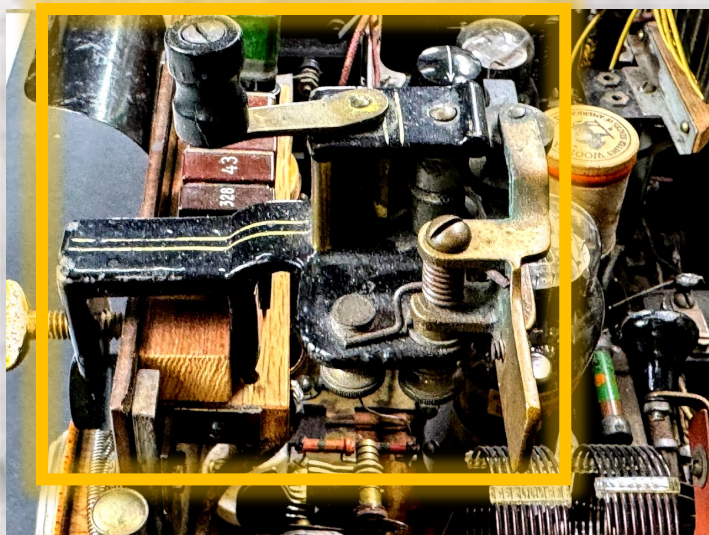
Nestled at the top right of the radio (as viewed from the front) is the Learners AA Morse Code tape reader and crank assembly
