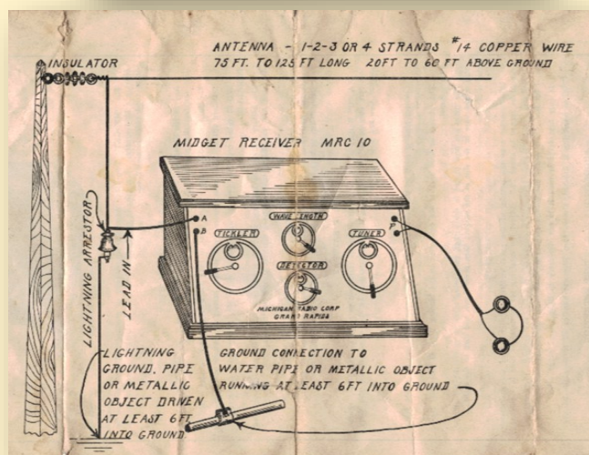
Klitzen MRC-10 instructions manual. To see full-size and zoomable simply right click > open new tab.
