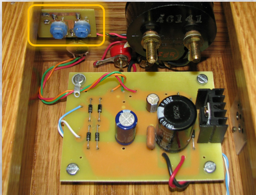
Mounting of the PC boards. Inset: the tiny PCB used to mount the trimmer pots
