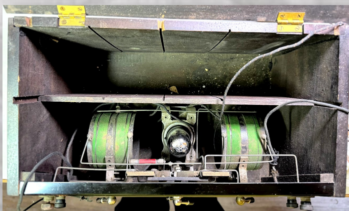
Inside view of the Klitzen receiver. The single CX-12 tube is in the center. The green coil on the left is the tickler and the coil on the right is the tuning coil. Both are variometer types.
