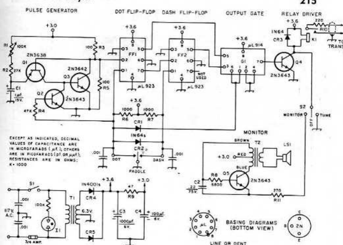
Fig. 7-10—Schematic of the MicroTO keyer. Capacitances are in \mu F, polarity indicates electrolytic, others are ceramic. Resistances are in ohms ( K = 1000 ); resistors are 1/2-watt. Component designations not listed below are for identification in board layout.
