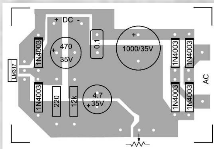
Simple PC Board Layout
