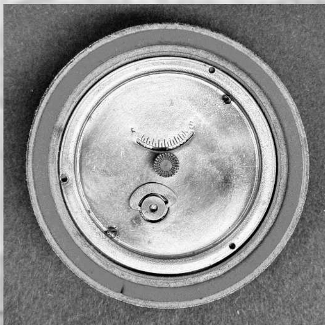
Rearview of the clock, showing time tracking adjustment and winder key
