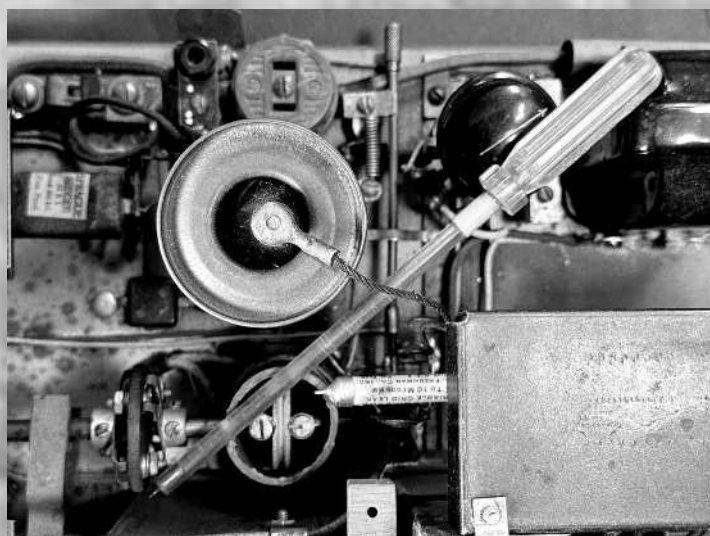
Semi-homebrew insulated screwdriver for ad- justing the receiver trimmers and tuning slugs
