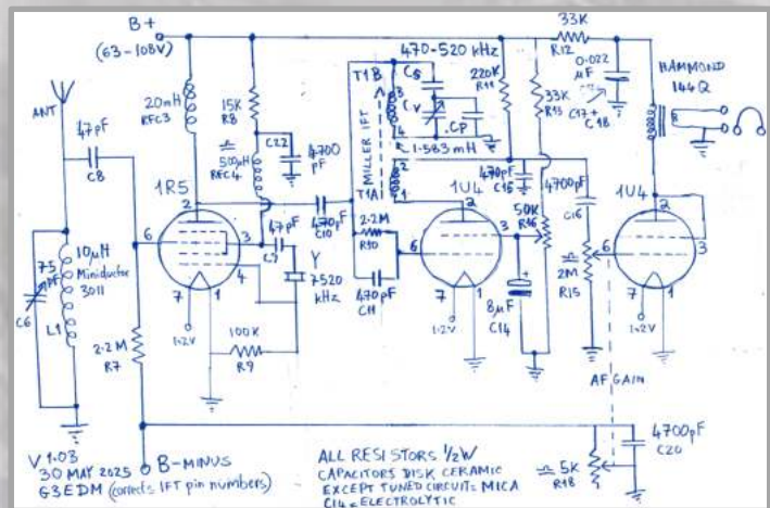
Three-tube superhet for 40-meters as built by Martin G3EDM for his Peashooter rig.
