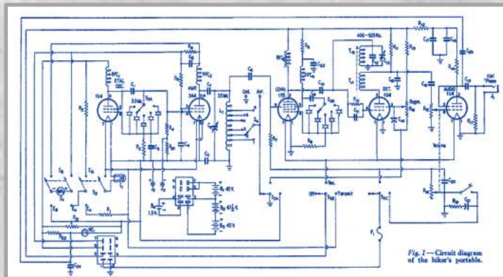
The original “Hiker’s Portable” from QST, September 1950. Martin adapted this circuit, eliminating as much unnecessary circuitry as possible to reduce the weight.
