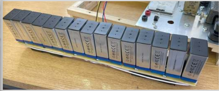
15 type PP3 Lithium-Ion "9v" (actually 8.7v) batteries in series
