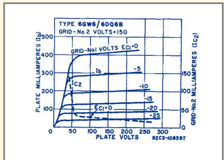
Typical RCA Tube Manual “curve tracer” graph
