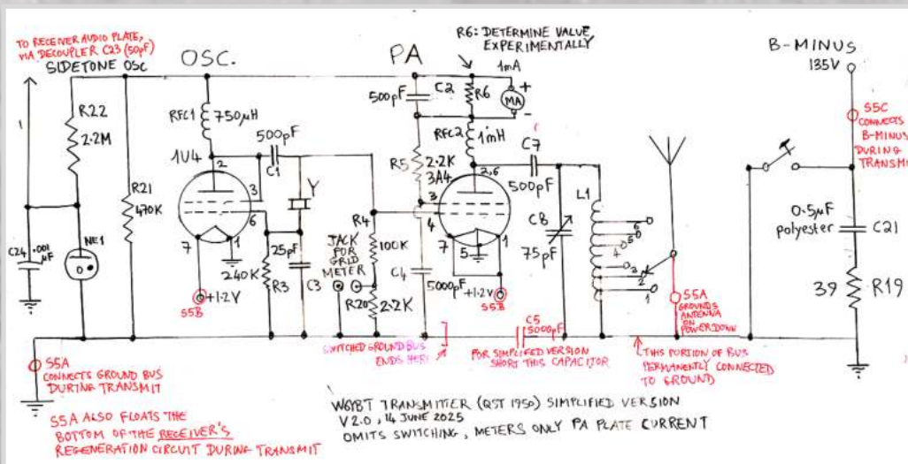
The 2-tube transmitter as adapted from the original by Martin G3EDM. The multi-tap tank coil helped greatly during his hike in dealing with varying antenna matching challenges.
